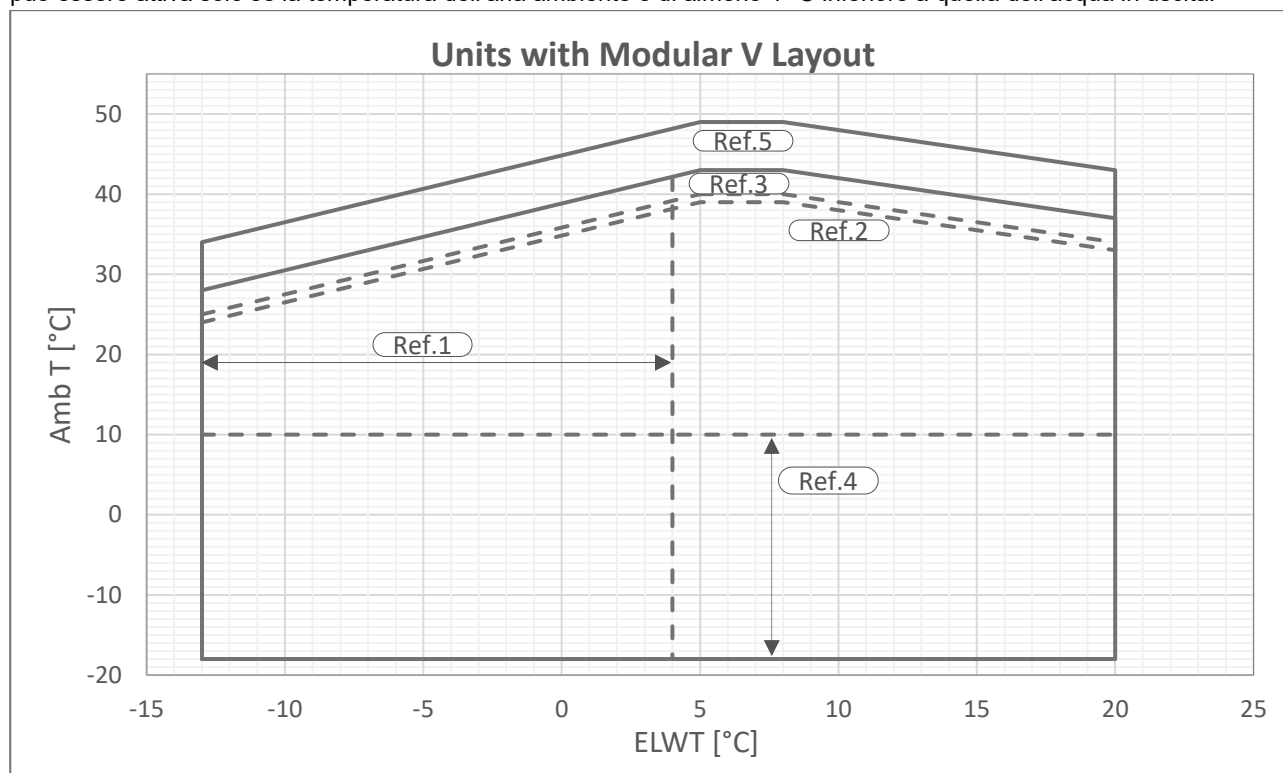
Fig. 9 - Limiti Operativi Multi V-Silver
