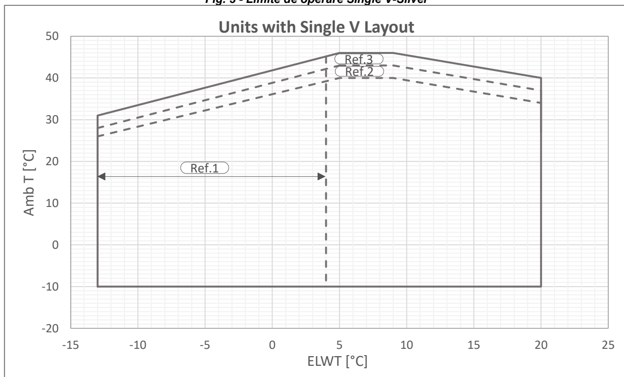
Fig. 4 - Limite de operare Single V-Gold
