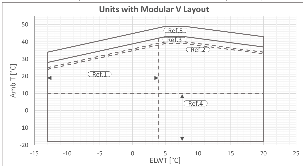
Fig. 1 - Limiti Operativi Multi V-Silver
