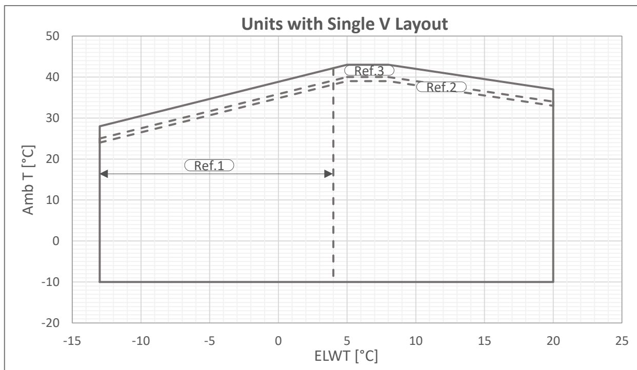
Fig. 3 - Limiti Operativi Single V-Silver
