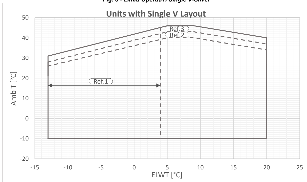
Fig. 4 - Limiti Operativi Single V-Gold
