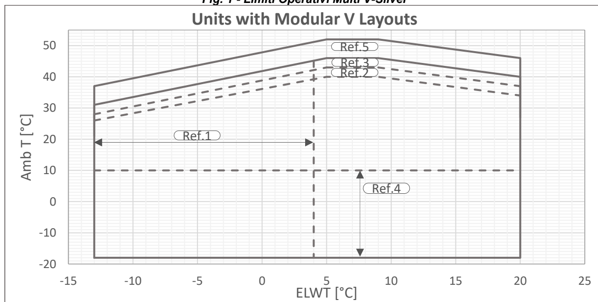
Fig. 2 - Limiti Operativi Multi V-Gold
