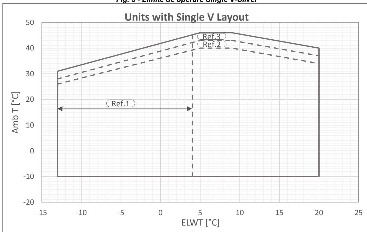
Fig. 4 - Limite de operare Single V-Gold
