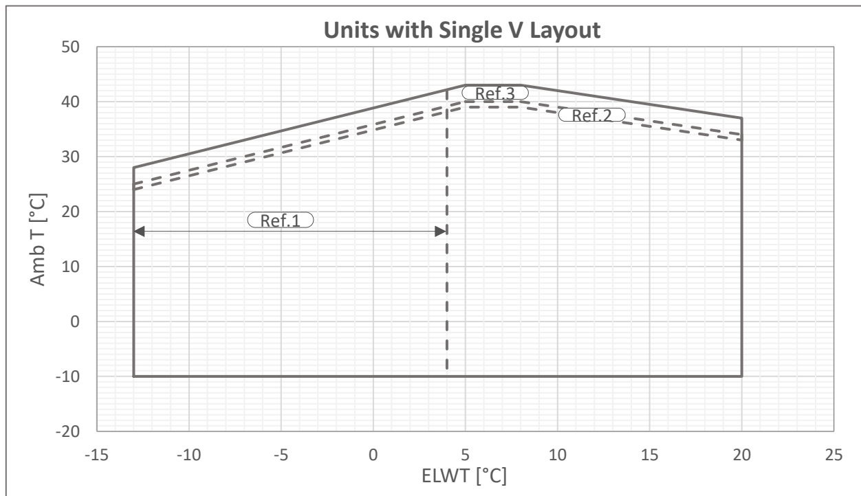
Fig. 8 - Limiti Operativi Single V-Gold
