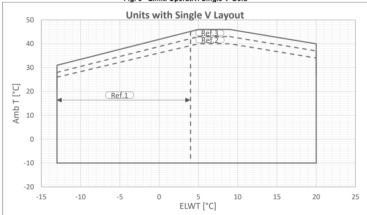
Fig. 8 - Limiti Operativi Single V-Gold
