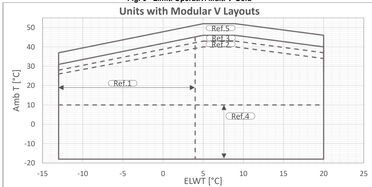
Fig. 6 - Limiti Operativi Multi V-Gold
