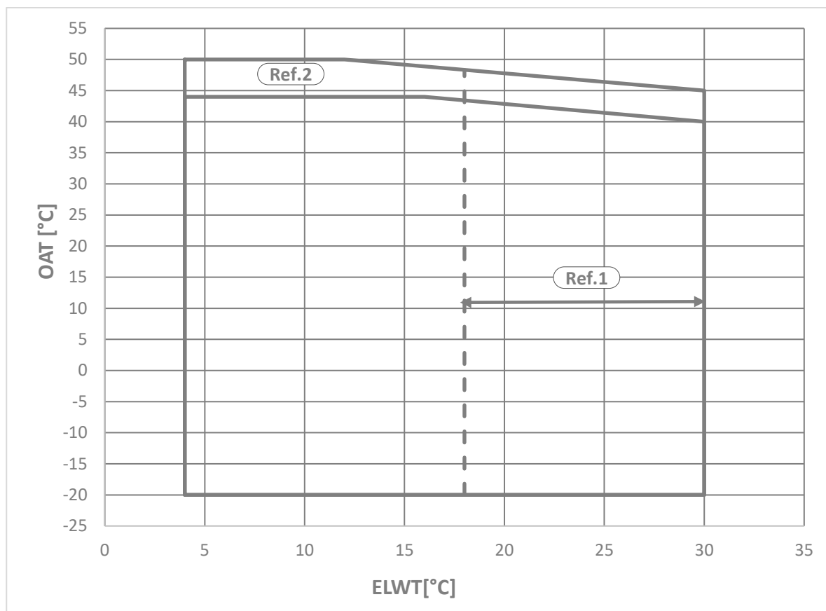
Fig. 7– EWFT-B-C Gold Operational limits
