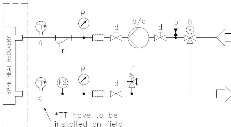
Slika 26- Water piping connection for Heat Recovery Exchangers (Maximum pressure 20 bar)
