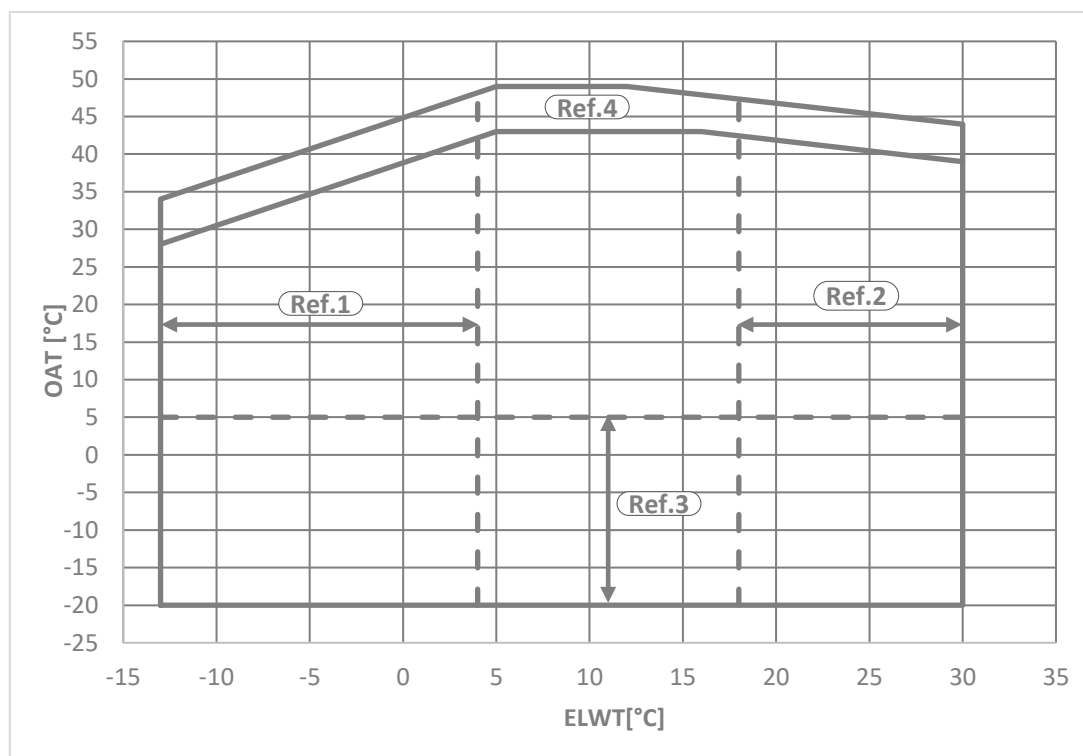
Fig. 4– EWAT-B-C Limite de operare Silver
