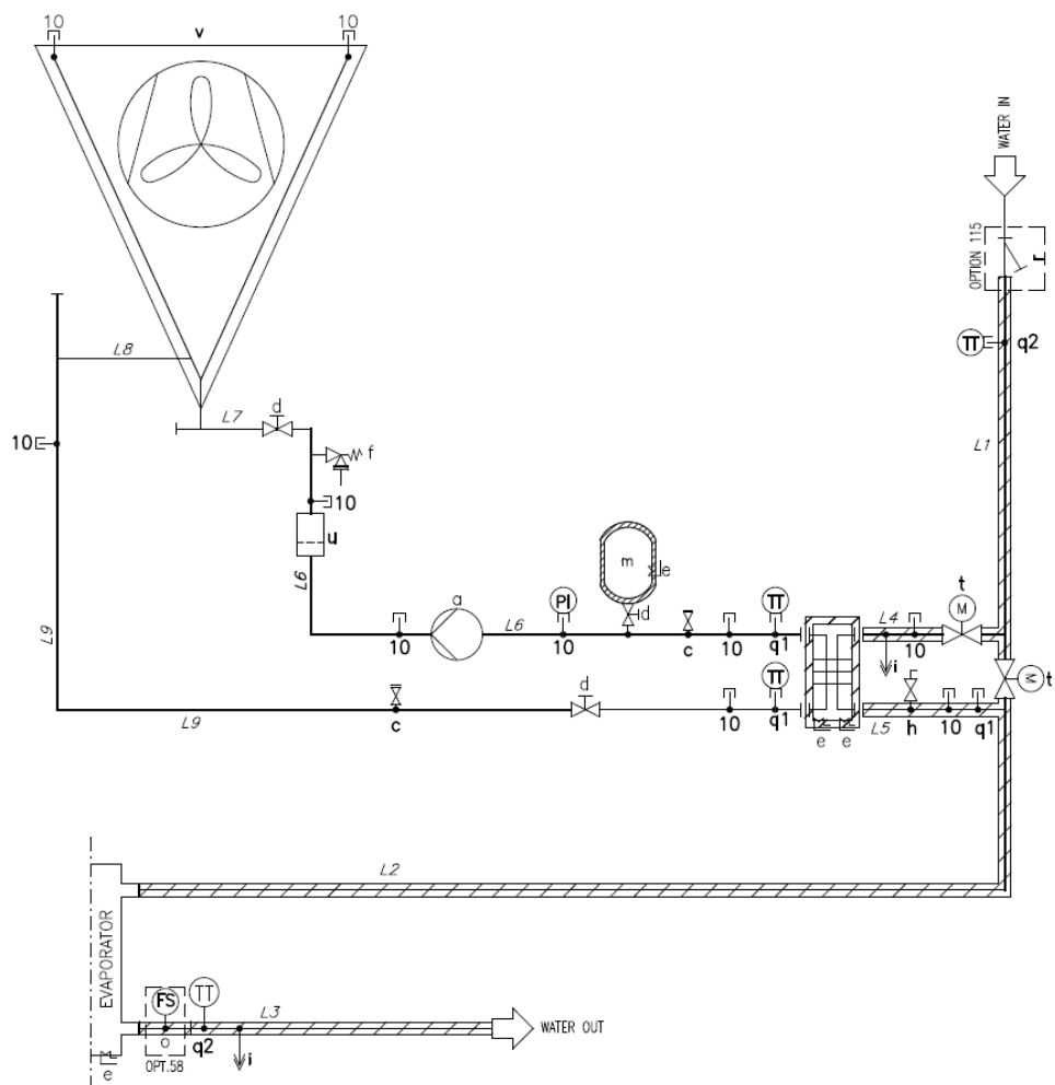
Obr. 27 - Uzavretá slučka Hydronic Free cooling P&ID (Opt. 231)
