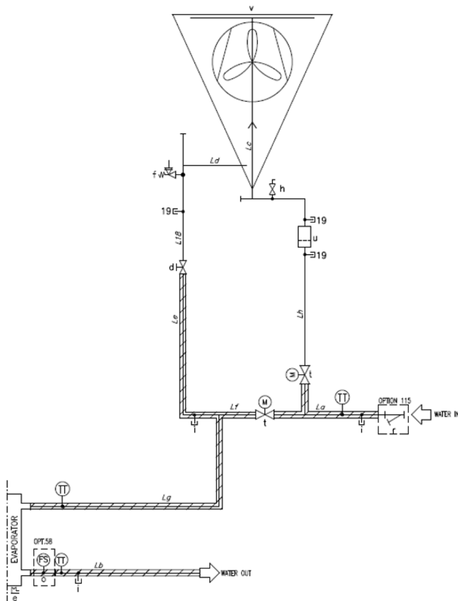
Fig. 28 – Hydronic Free cooling P&ID
