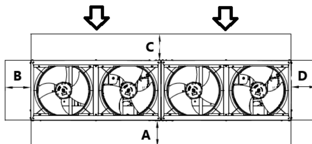
Illustration 6 – Unité DUAL
