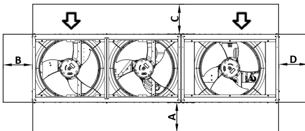
Figure 9 – unité DUALE
