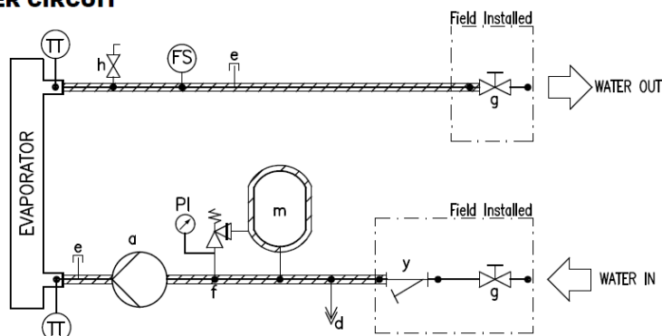
WATER CIRCUIT
