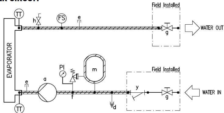
WATER CIRCUIT
