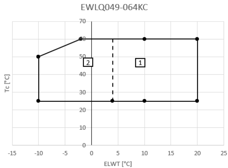
Figura 4-EWLQ049-064KC
