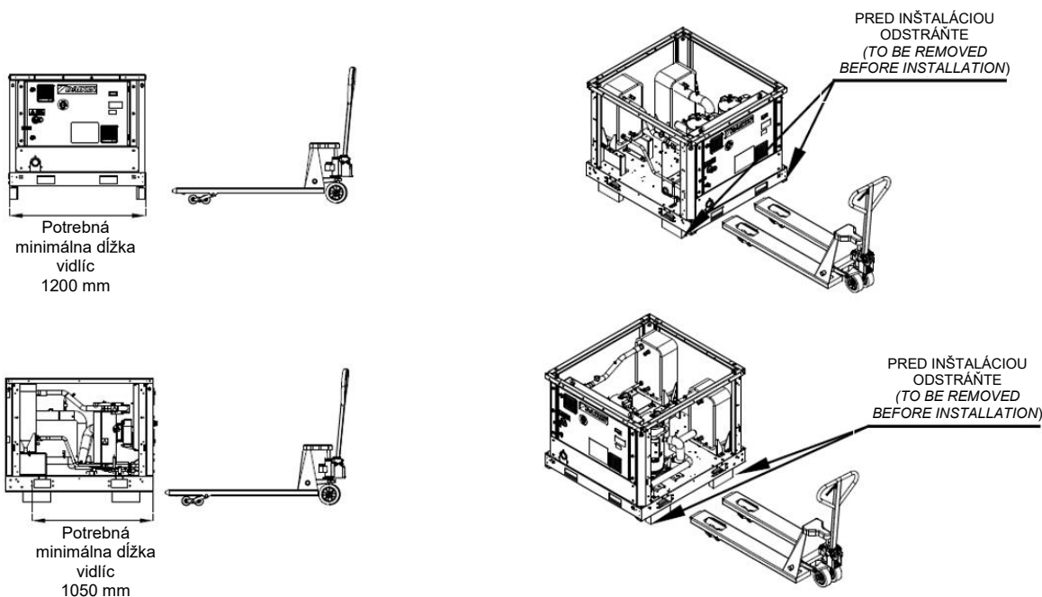
Obr. 13 – Alternative handling method with pallet truck
