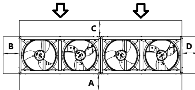
Figure 8 – Unité DUAL
