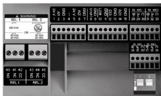
Figure 13 - Plaque à bornes HydrovarX EXM
