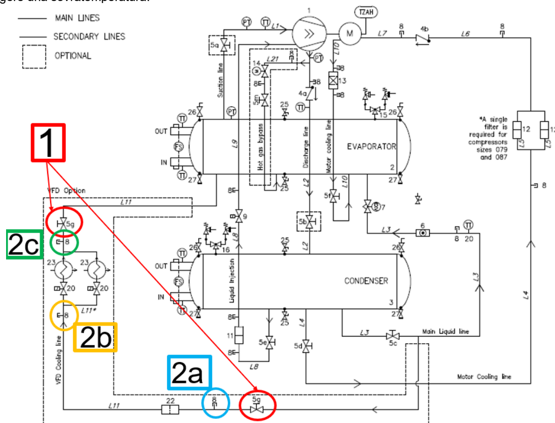
Fig.° 26- P&ID diagram of the unit with inverter cooling line detail
