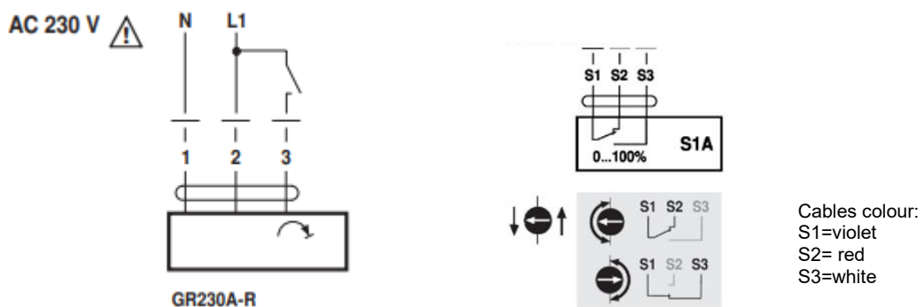
Fig. 11 – Wiring diagram for motor (left figure) and limit switches (right figure)
