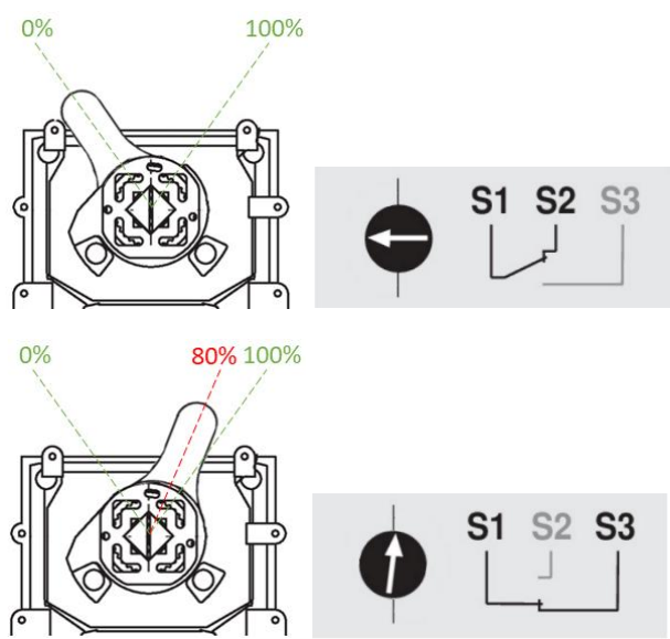
Fig. 18 – Setting of limit switches trigger
