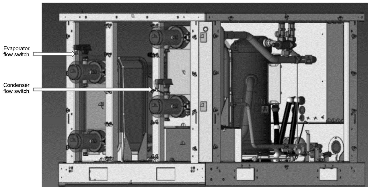
Fig. 3– Cables routing of evaporator flow switch
