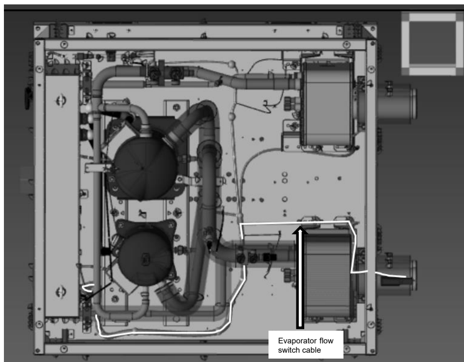
Fig. 4 – Cables routing of evaporator flow switch
