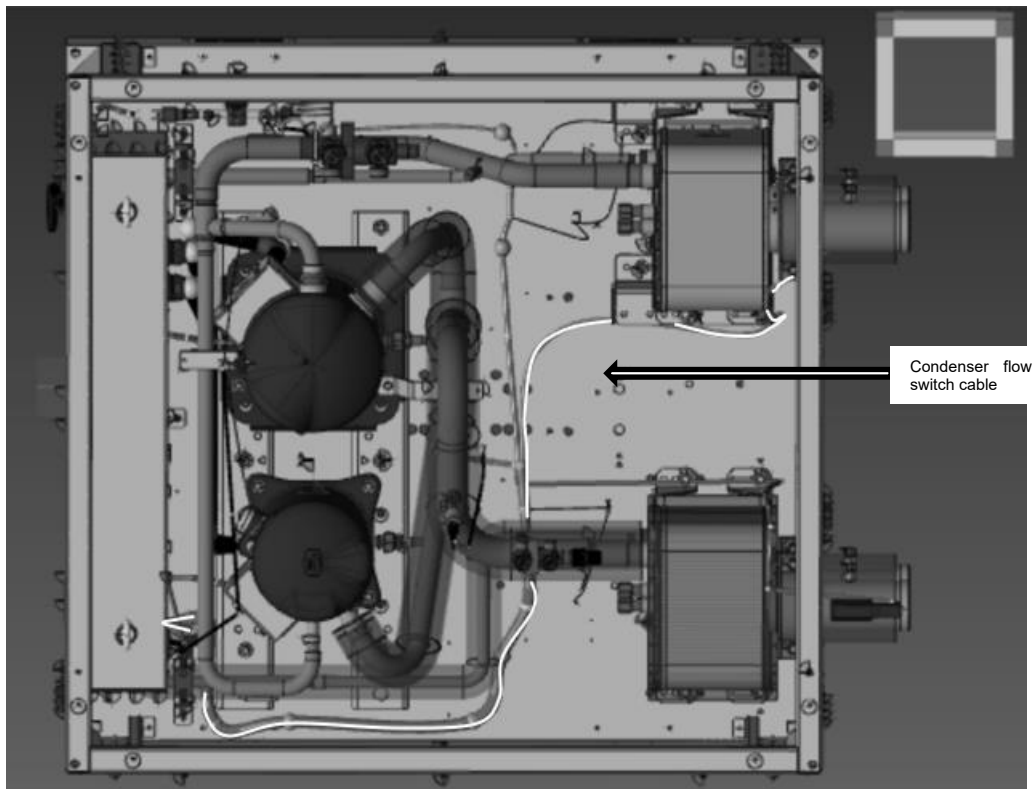
Fig. 5 – Electrical panel entry point for evaporator and condenser flow switch cables
