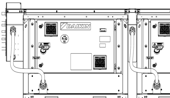
Fig. 21 – Details of cables routing
