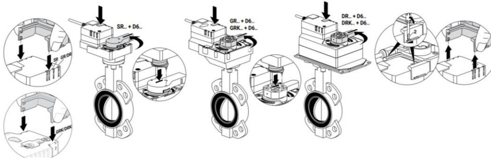
Fig. 9 – Mounting instructions for actuator limit switches
