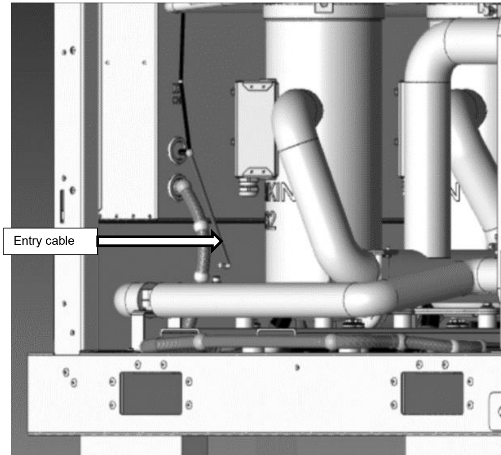
Fig. 17 – Electrical panel entry for evaporator and condenser shut off valve actuator cables
