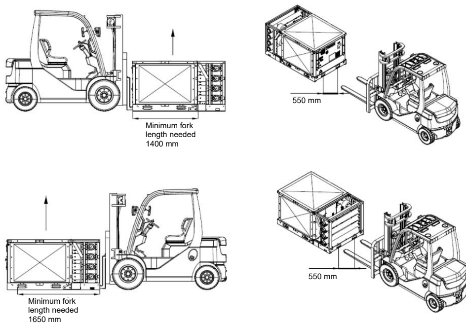
Fig. 34 – Handling of unit and manifold modules (1)
