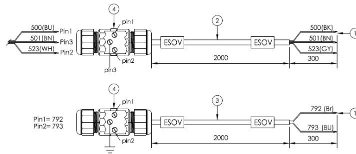
Fig. 13 – Cable adapters for condenser shut off valve actuator and limit switches
