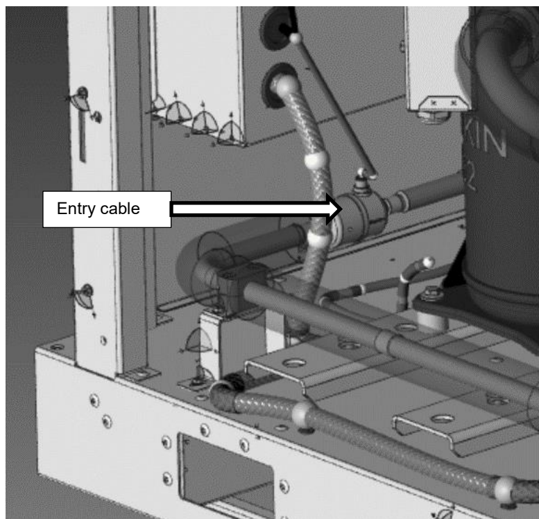
Fig. 5 – Electrical panel entry point for evaporator and condenser flow switch cables
