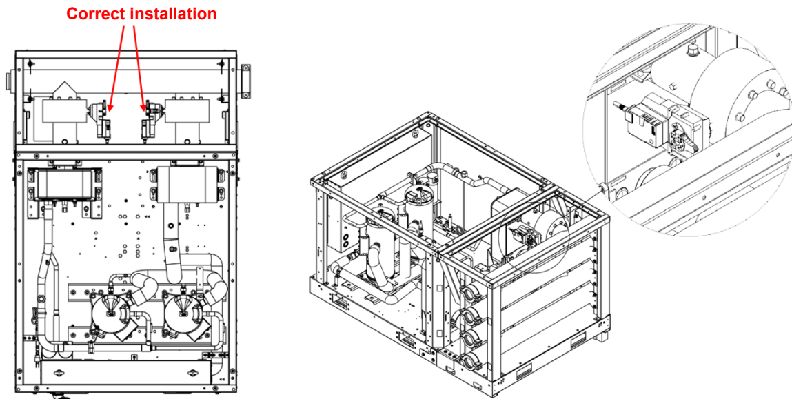
Fig. 10 – Mounting indications for valve actuator
