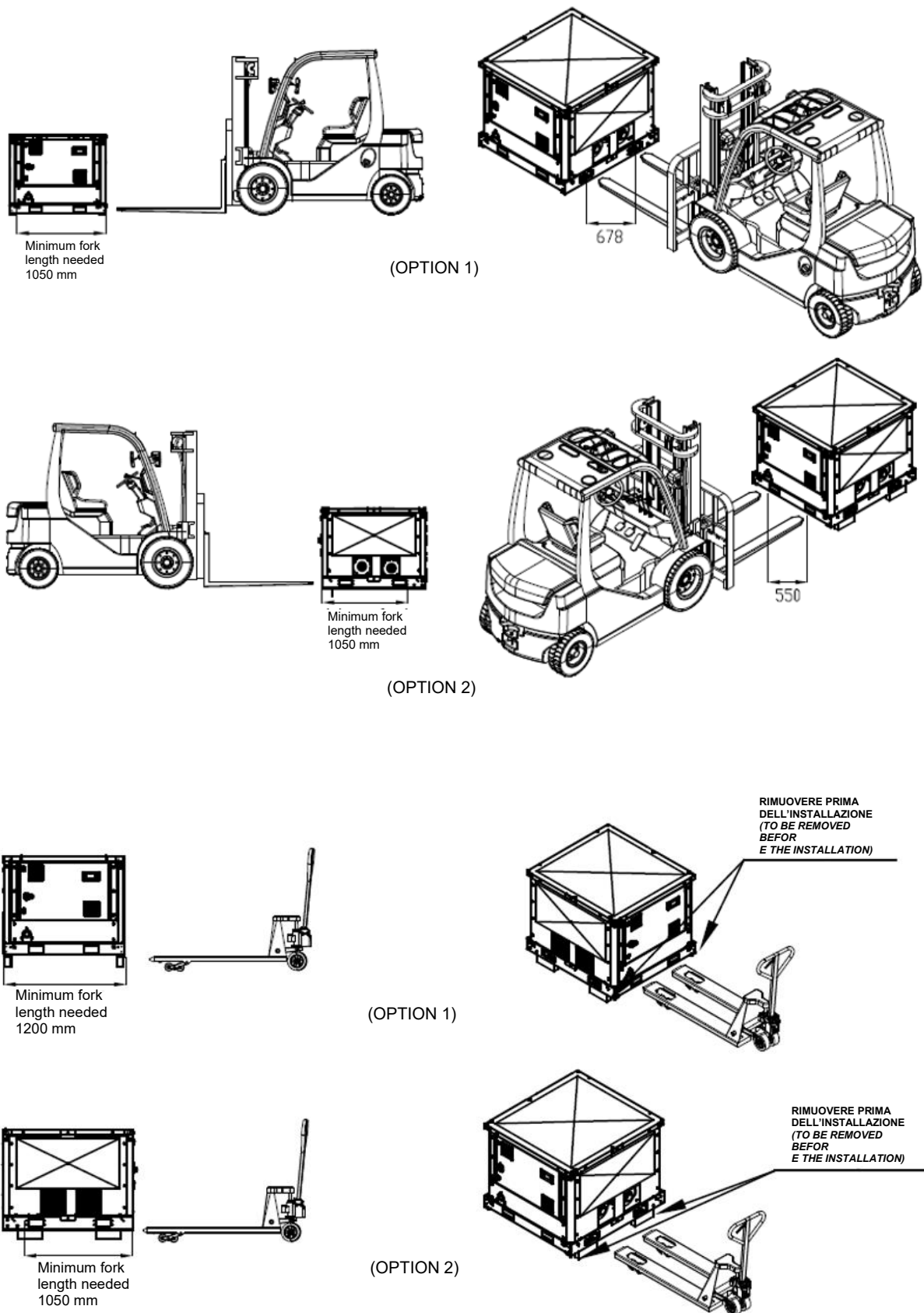
Fig. 29 – Handling of pump module
