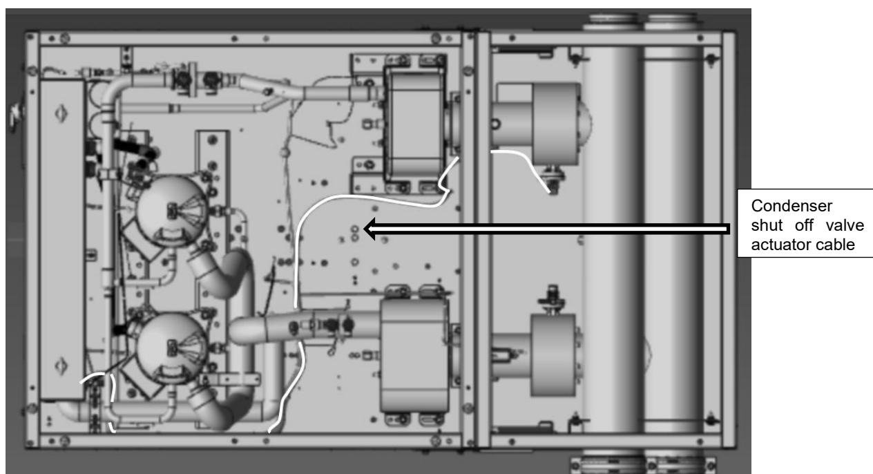
Fig. 16 – Condenser shut off valve actuator cable routing
