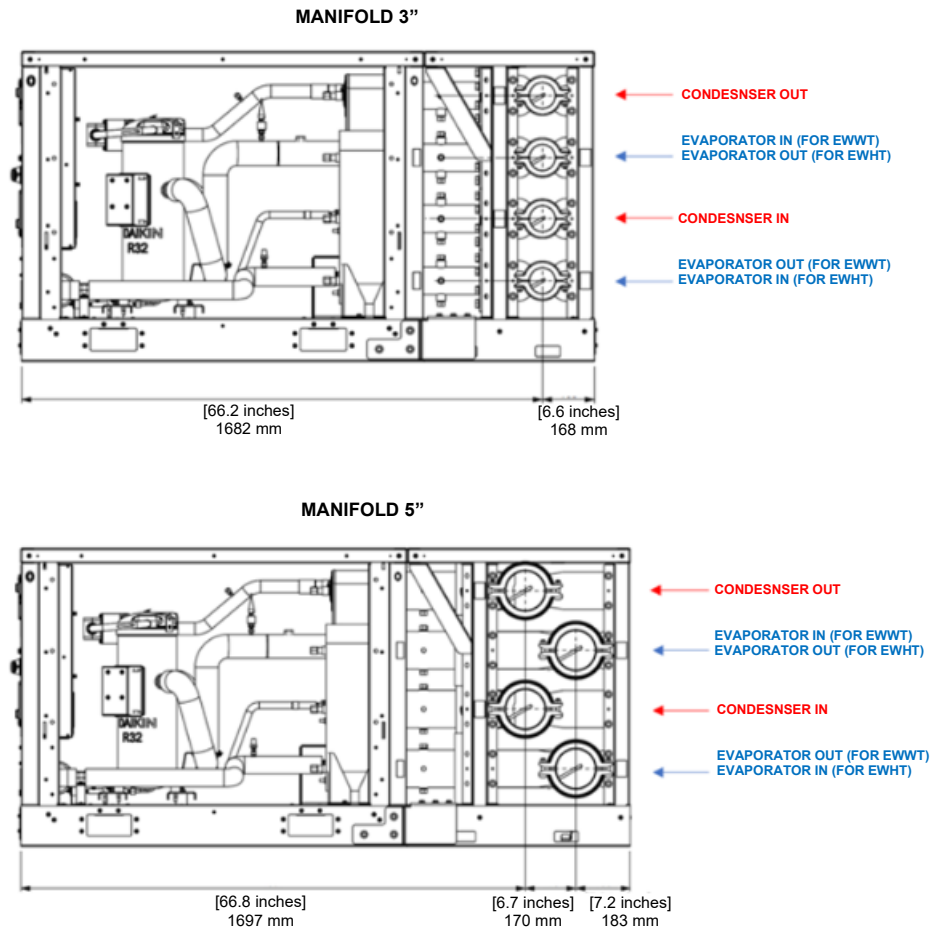
Fig. 31 – Water manifold sizes
