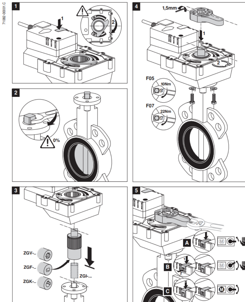
Fig. 8 – Mounting instructions for valve actuator
