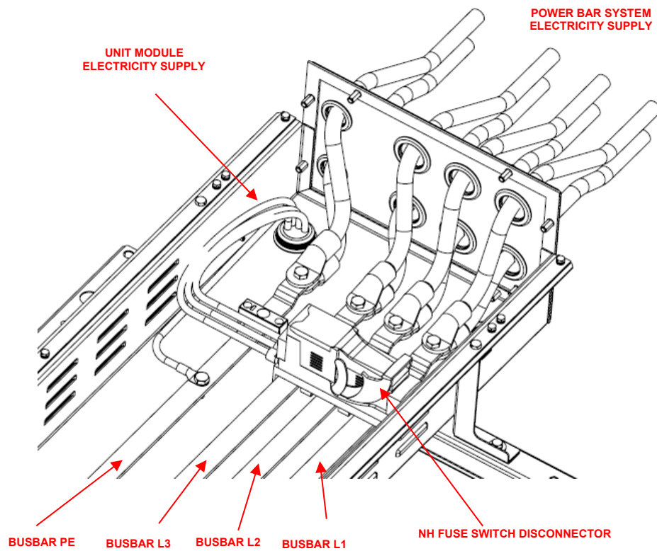
Fig. 27 – Detail of electrical connection for any other unit module
