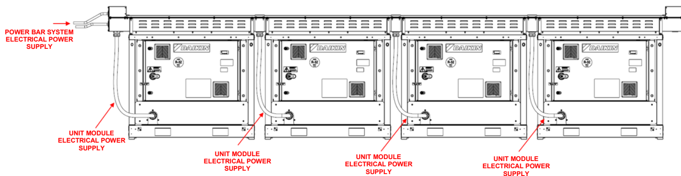
Fig. 21 – Details of cables routing
