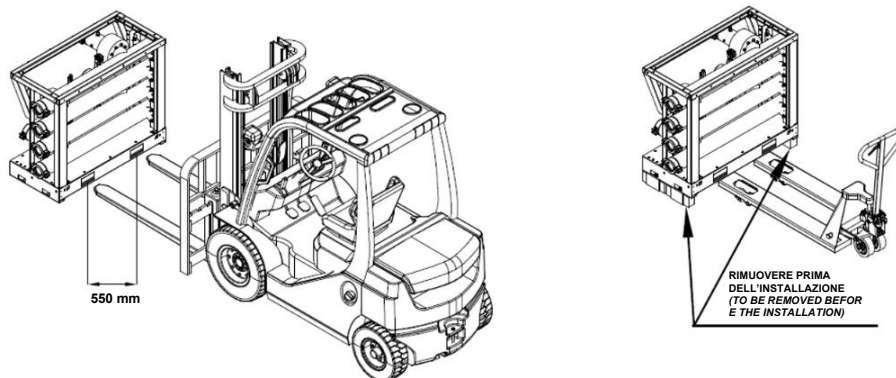
Fig. 33 – Handling of manifold module
