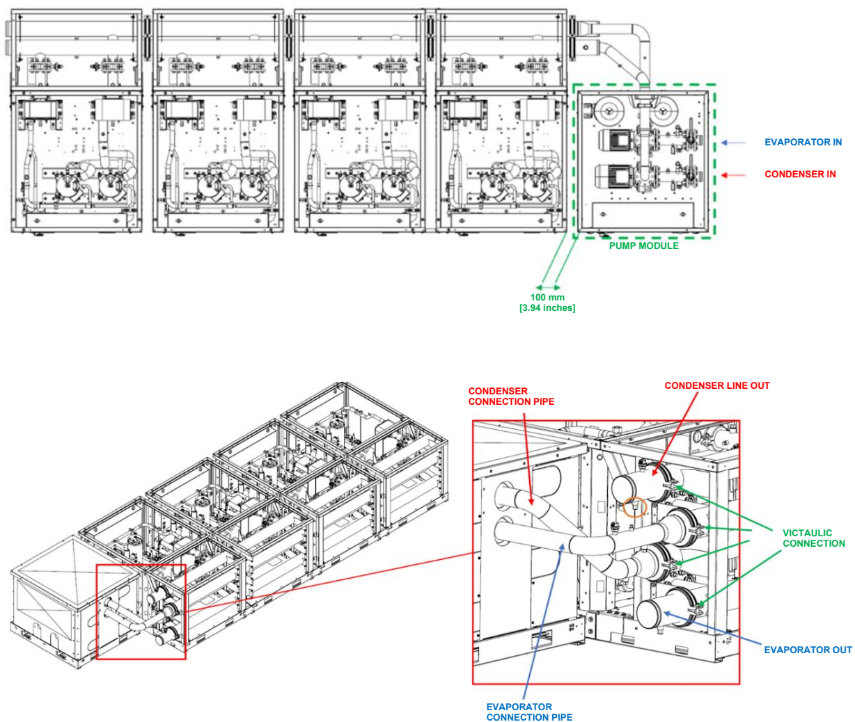
Fig. 28 – Pump module installation
