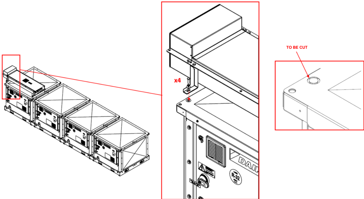
Fig. 22 – Fixing of the power bar system to the unit
