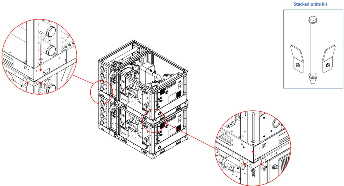
Fig. 6 – Mounting instructions for stacked units
