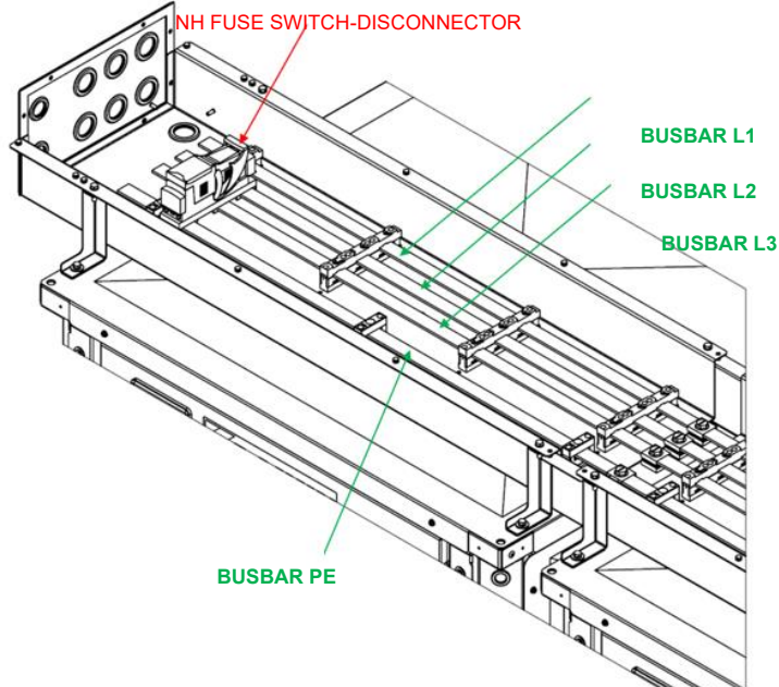
Fig. 25 – Detail of the fuses and of the box for cables routing of the power bar module
