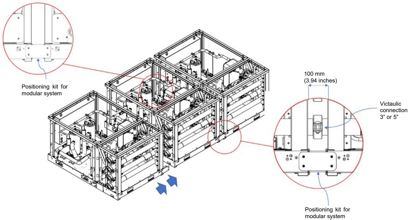
Fig. 7 – Modular systems connection
