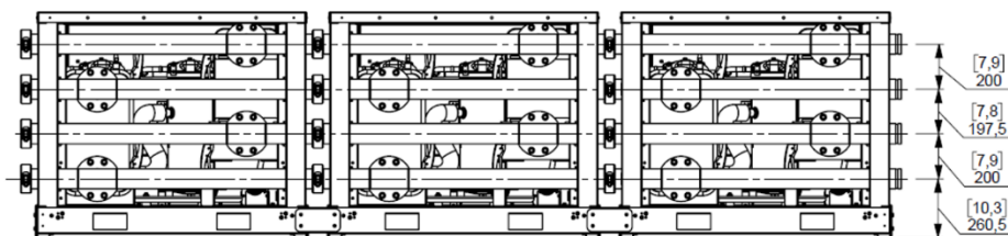
Fig. 32 – Water connection to modules
