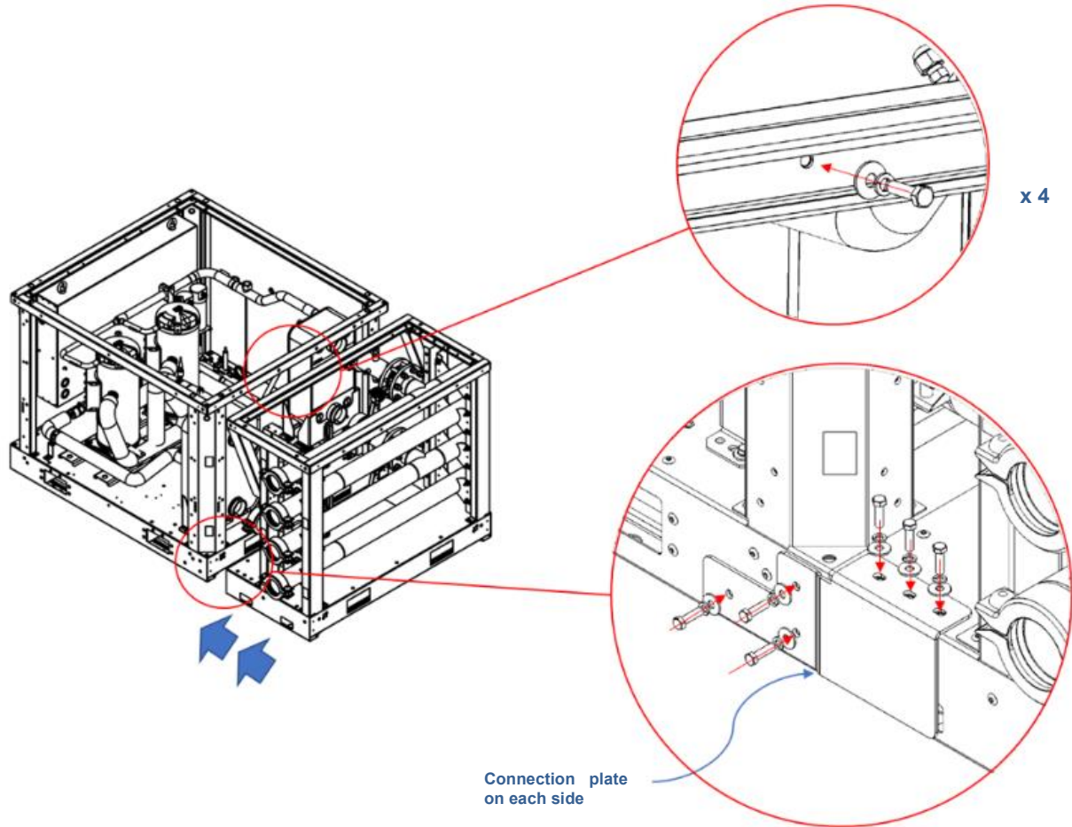
Fig. 30 – Connection instructions between chiller and manifold modules
