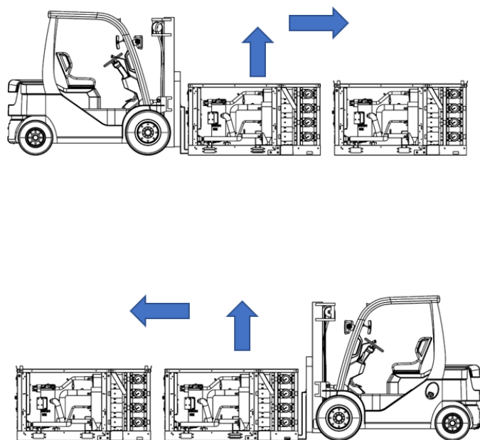
Fig. 35 – Handling of unit and manifold modules (2)
