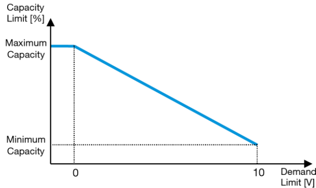
Grafico 2 – Demand Limit[V] vs Capacity Limit[%]
