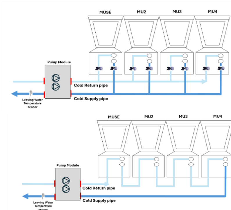
MUSE Parallel Vs Series Configuratieschema's
